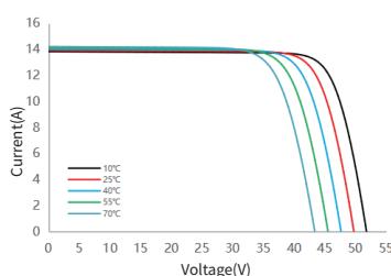
I-V Curve at Different Temperature SS8-72HD-545M
