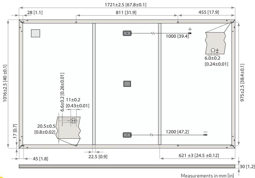
Fig. 19: Panel dimensions: REC Alpha Series
