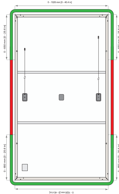
Fig. 24: REC Alpha 72 Series MLPE device installation zones
