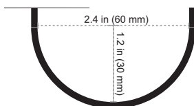
Fig. 18: Minimum cable bend radius
