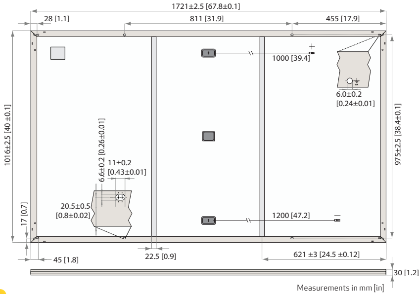
Fig. 20: Panel dimensions: REC Alpha Black Series
