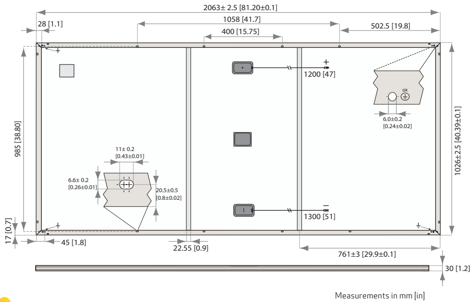
Fig. 22: Panel dimensions: REC Alpha 72 Series
