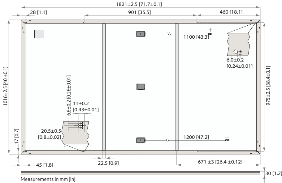
Fig. 21: Panel dimensions: REC Alpha Pure Series
